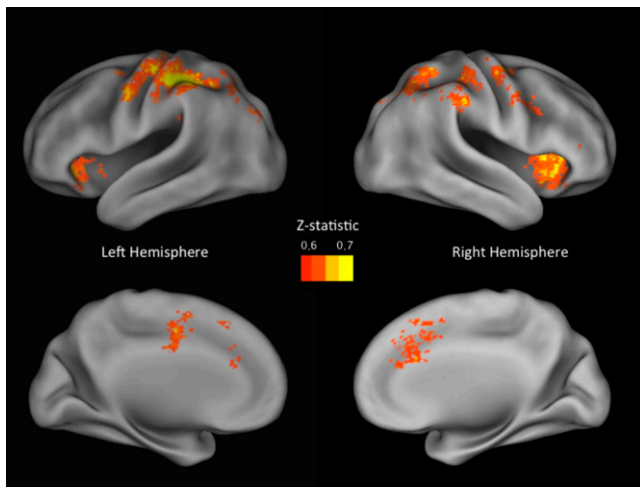
Fig. 2. Classification searchlight analysis of pre-cash out vs. prepump trials. Colored voxels indicate centers of searchlights where the classifier could successfully discriminate between prepump and pre-cash out activation patterns (searchlight classification >60%, whole-brain cluster-corrected P < 0.05 via comparison with 1,000 random permutations). (Scale: 60–70%.) Activation maps were projected onto an inflated average cortical surface of the Population-Average, Landmark-, and Surface-Based (PALS) atlas using the multifiducial mapping technique of Van Essen (29).
