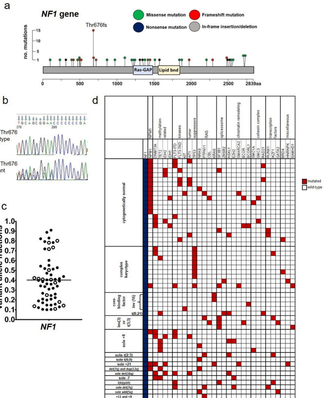
Figure 1. Mutations in the NF1 gene found in 1,021 patients with de novo acute myeloid leukemia. (a) Lollipop plots depicting 59 NF1 mutations detected in 52 patients. No. denotes number; aa, amino acid. (b) Sanger sequencing traces depicting examples of NF1 amino acid Threonine (Thr) 676 wild-type (top) and mutated (bottom) AML cases. (c) Beehive plot depicting variant allele fractions of the detected NF1 mutations. (d) Oncoprint of co-occurring mutations found in at least two AML patients with NF1 mutations (blue color), and of genes classified into the previously described functional groups. 11 Each column represents an
